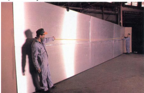
Tank shell for the food processing industry made into one continuous piece using automatic splice welding prior to rolling.
