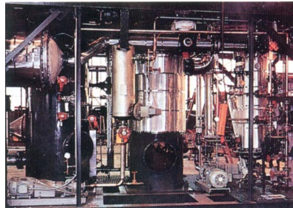
Skid-mounted formaldehyde production plant for the chemical industry completely assembled within our fabrication facility.
