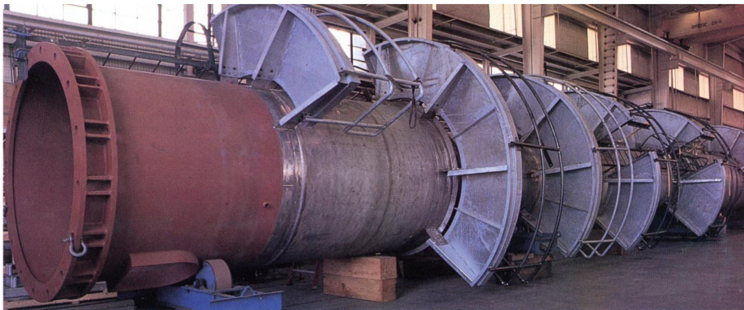
Extractor tower, 90" diameter x 1/2" wall x 83 ft. high with prefit platforms, fabricated from Type 304 stainless steel for the petrochemical industry.
