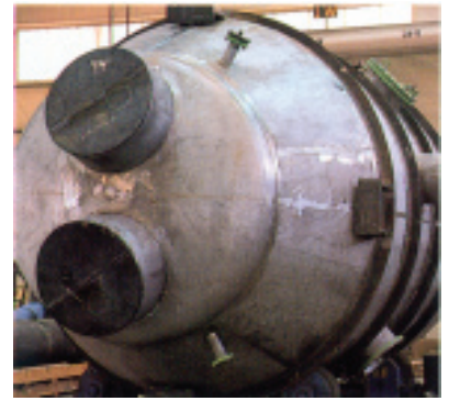
Stainless steel concentrator vapor head, over 11 ft. in diameter.
